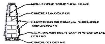
TYP. ANCHORAGE NOT TO SCALE
